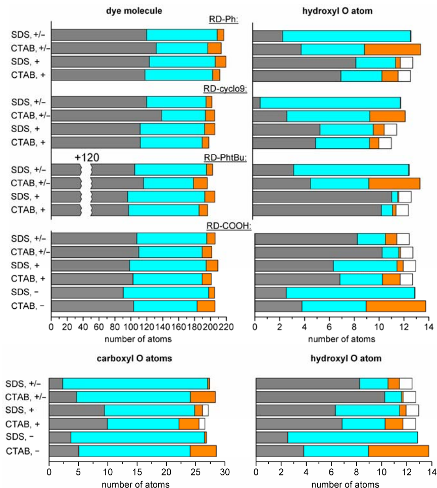
Figure 6. Average numbers of atoms of three categories in the microenvironment of the whole dye molecule and its O atoms. The sections of bars correspond to (left to right): the micelle core atoms (gray), the water atoms (cyan), the headgroup atoms (orange), the covalently bonded H atom (white). The microenvironment of the RD-COOH hydroxyl O atom is shown twice for convenience. The data for RD-Ph are from ref. [9].
