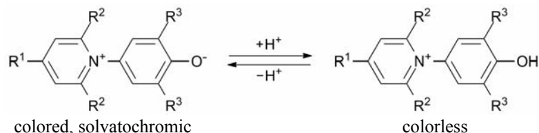
Figure 1. Molecular structure of solvatochromic pyridinium N -phenolate dyes.
